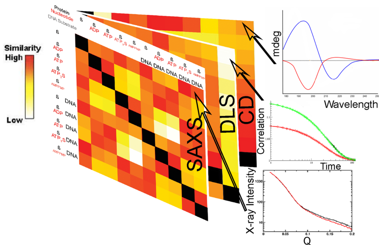
Figure 1. Heat map comparing pairs of profiles from multiple experimental techniques including SAXS, DLS, and CD. Each cell is a pairwise comparison between a condition or construct. Similarity between SAXS curves is measured by the metric V_r and displayed as a gradient color, where red indicates similarity (low V_r score) and white indicates dissimilarity. The black square diagonals are self-comparisons. Adapted with permission from ref 79. Copyright 2016 Nature Publishing Group.
