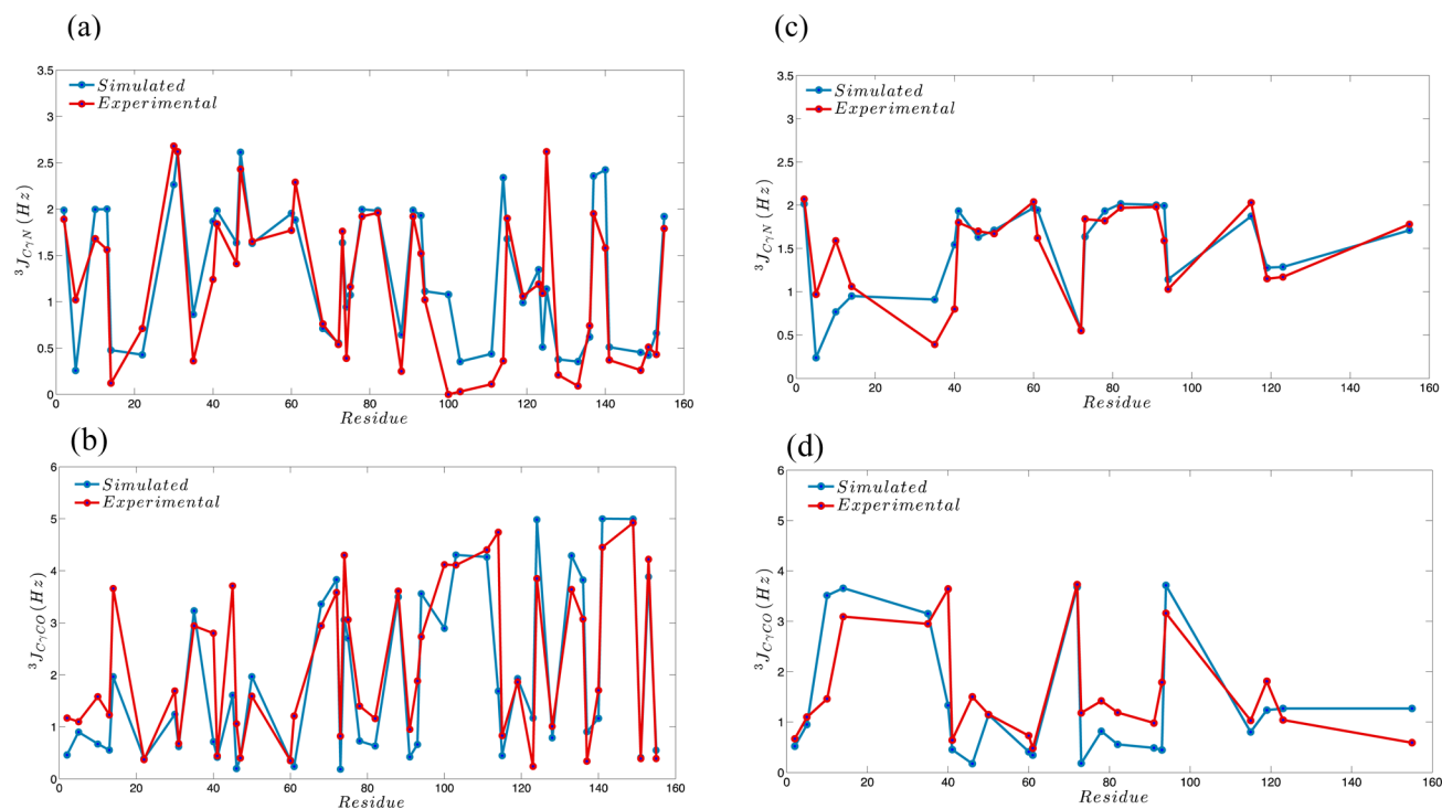
Figure 4. J -coupling constants: (a) {}^3J_{C7N} and (b) {}^3J_{C7CO} for the DHFR binary product complex E:THEF, and (c) {}^3J_{C7N} and (d) {}^3J_{C7CO} for the DHFR binary product complex E:FOL. The red symbols are the experimental data from ref 167. The blue symbols are calculated from the MC-SCE ensemble using backbones from molecular dynamics and the Karplus parametrization from ref 167. Reprinted with permission from ref 61. Copyright 2015 Elsevier.
