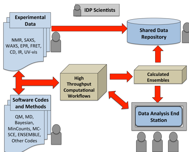
Figure 5. Conceptualization of a computational beamline for the IDP community.
