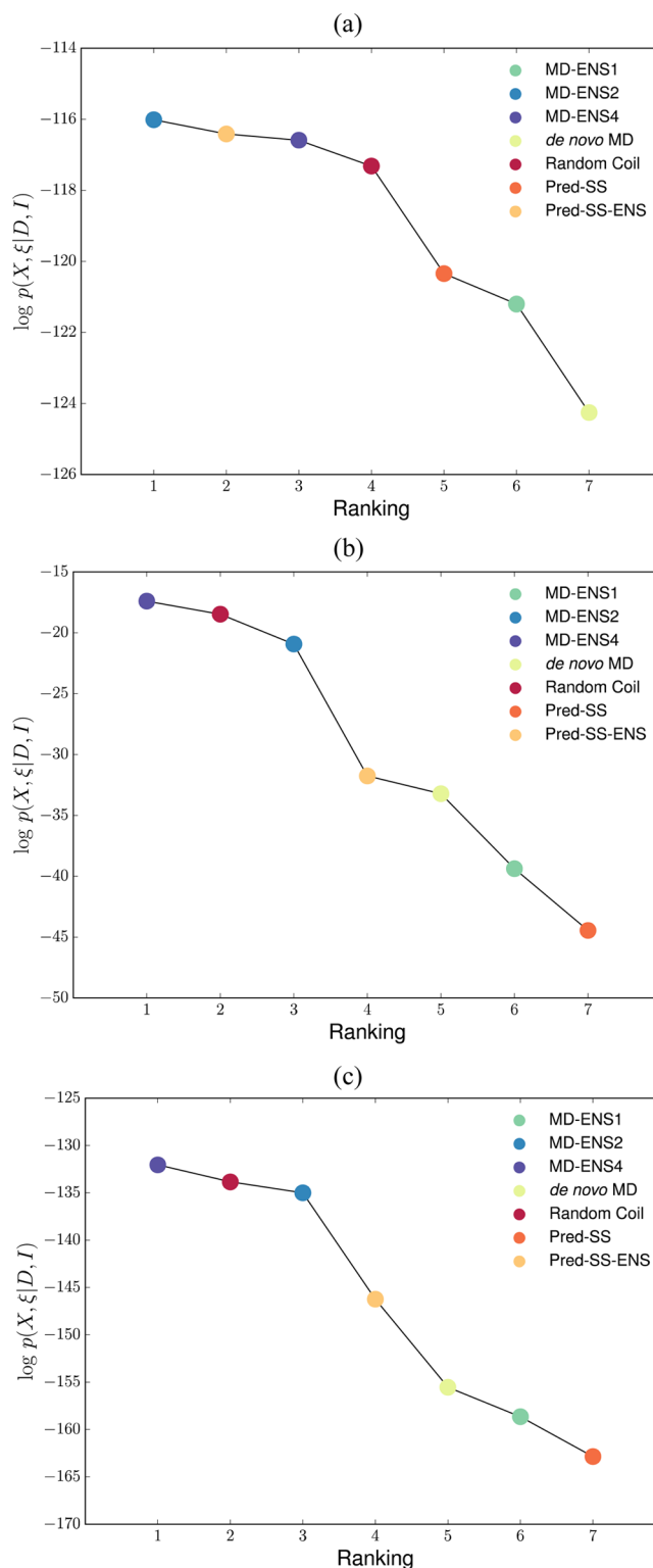
Figure 2. \log p(X, \xi|D, I) evaluated for X equal to the following qualitatively different ensembles for the A \beta 42 monomer: random coil (RC), statistical secondary structure (Pred-SS), de novo MD, and ENSEMBLE optimized ensembles (MD-ENS1, MD-ENS2, MD-ENS4, and Pred-SS-ENS) using (a) chemical shift data only, (b) J -coupling data only, and (c) J -coupling and chemical shift data together. Adapted with permission from ref 62. Copyright 2016 American Chemical Society.
