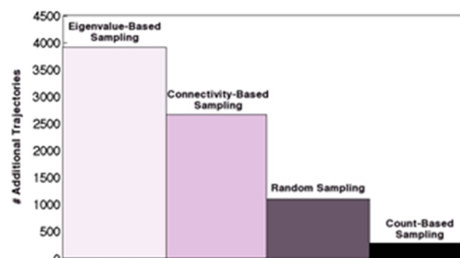
Figure 3. Convergence time for Fs (capped 21 alanine) peptide transition matrix generated with various hybrid sampling schemes. Time is measured in the number of eigenvalue-based trajectories needed to converge to an absolute error of 2.00 after 1000 initial trajectories are run from a chosen sampling method. Absolute error is defined as the sum of absolute deviations in transition matrix elements. Convergence times for each method were, averaged over 10 simulations, (1) 3913 for pure eigenvalue-based sampling, (2) 2669 for connectivity-based hybrid sampling, (3) 1107 for even sampling hybrid sampling, and (4) 286 for min count-based hybrid sampling. Reprinted with permission from ref 154. Copyright 2011 American Chemical Society.
